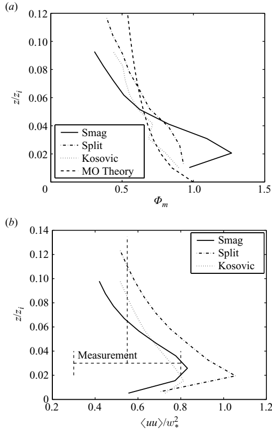
FIGURE 1. (a) LES results of the mean vertical gradient of the horizontal resolvable-scale velocity in the surface layer. The dashed line is the empirical form based on the the Monin–Obukhov similarity theory (Businger et al. 1971); (b) LES results of the horizontal velocity variance and the Minnesota measurements (Wyngaard 1988) with an error bar.
