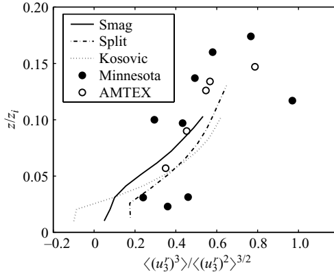
FIGURE 2. LES results of the vertical resolvability-scale velocity skewness profiles in the surface layer. The solid and open circles are from the Minnesota experiment (Wyngaard 1988) and AMTEX (Lenschow & Stephens 1980), respectively.
