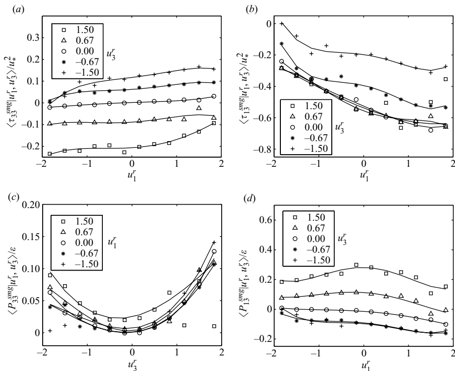
FIGURE 13. The Smagorinsky model results ( a posteriori test) of the conditional SGS stress and its production rate.
