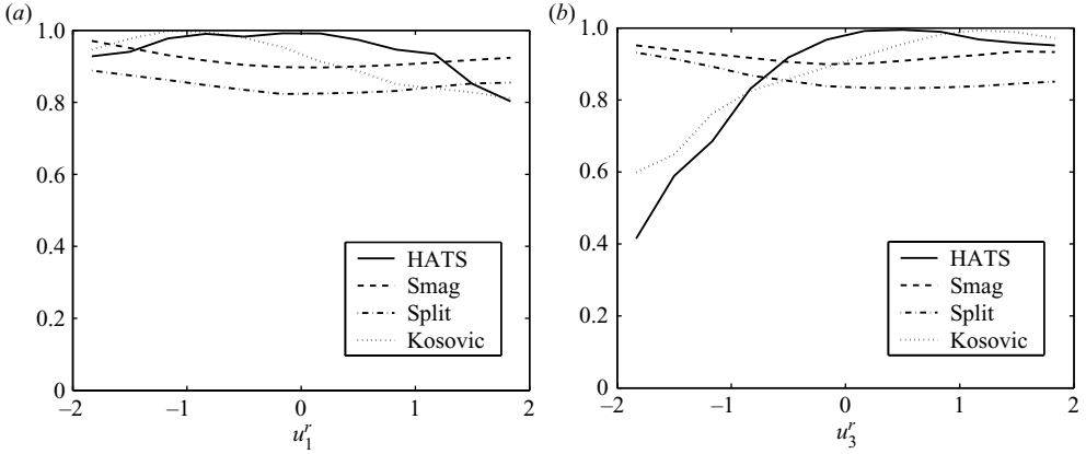
FIGURE 16. Contraction of the conditional SGS stress and its production rate from the LES ( a posteriori test) and the measurements.
