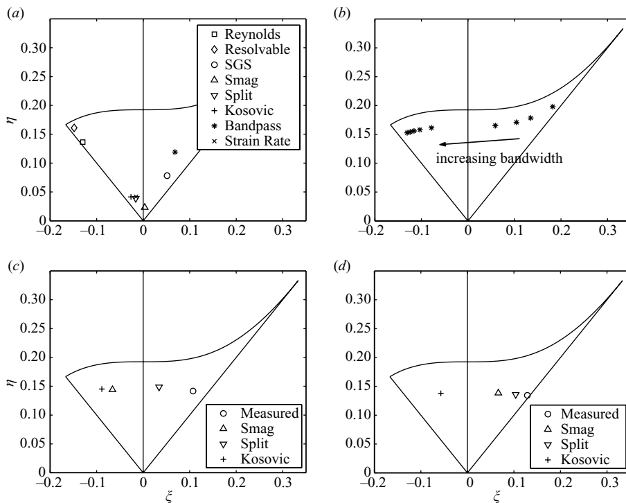
FIGURE 3. Lumley triangle representations of (a) the measured Reynolds stress, mean resolvable-scale stress, mean SGS stress, mean band-passed stress with a second filter size twice that of the first filter and the modelled ( a priori test) mean SGS stress. The strain rate is also given for reference. (b) the LES results of the mean band-passed stress using the Kosovic model. The bandwidth increases from 2 grid spaces to 34 grid spaces with an increment of 4 grid spaces; (c) the measured and the modelled ( a priori test) mean SGS stress production rate \langle P_{ij}^d \rangle ; (d) the measured and the modelled ( a priori test) \langle P_{ij}^d \rangle .
