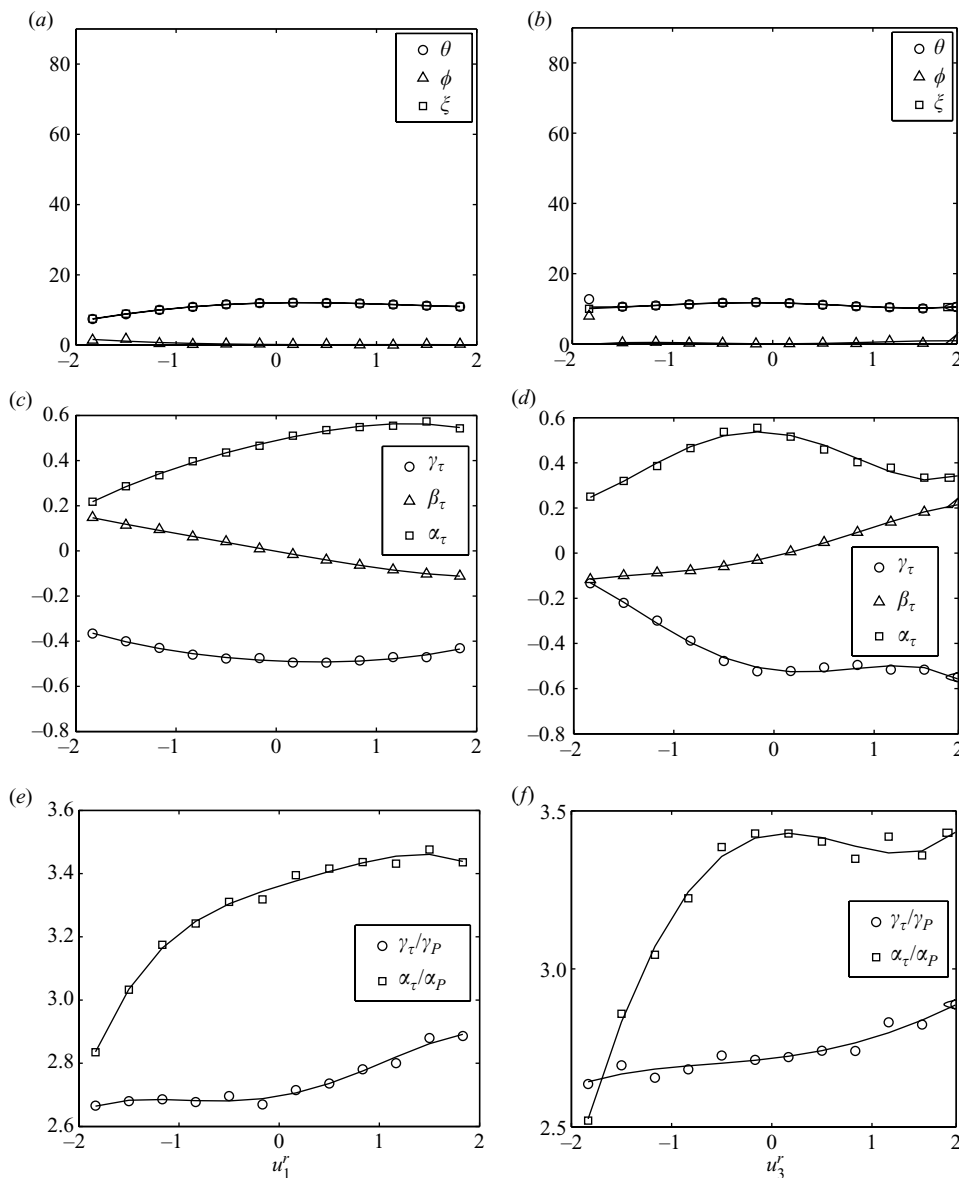
FIGURE 15. The Smagorinsky model results ( a posteriori test) of the geometric alignment angles and eigenvalues of the conditional SGS stress and its production rates ( a, b ) the geometric alignment angles; ( c, d ) the eigenvalues of the conditional SGS stress; ( e, f ) the eigenvalue ratios of the conditional SGS stress to its production rate.
