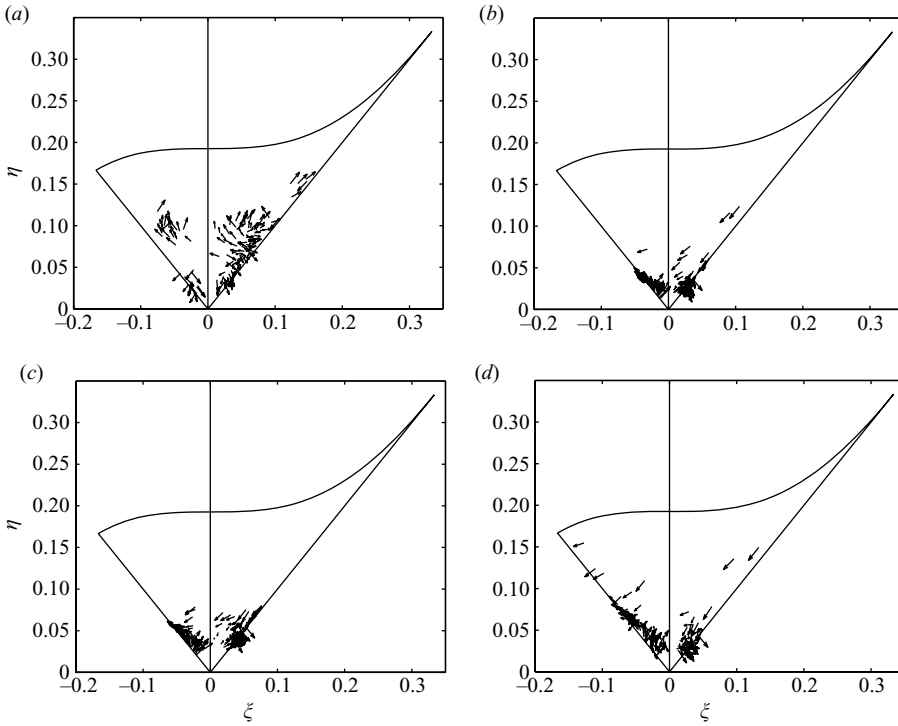
FIGURE 8. Lumley triangle representations of the measured and modelled ( a priori test) conditional SGS stress (a) the measurements; (b) the Smagorinsky model; (c) the split model; (d) the Kosović model. The arrows represent the conditioning vector (u_1^r, u_3^r) .
