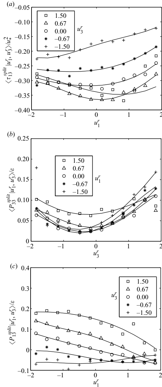
FIGURE 17. The split model results ( a posteriori test) of the conditional SGS stress and its production rate.
