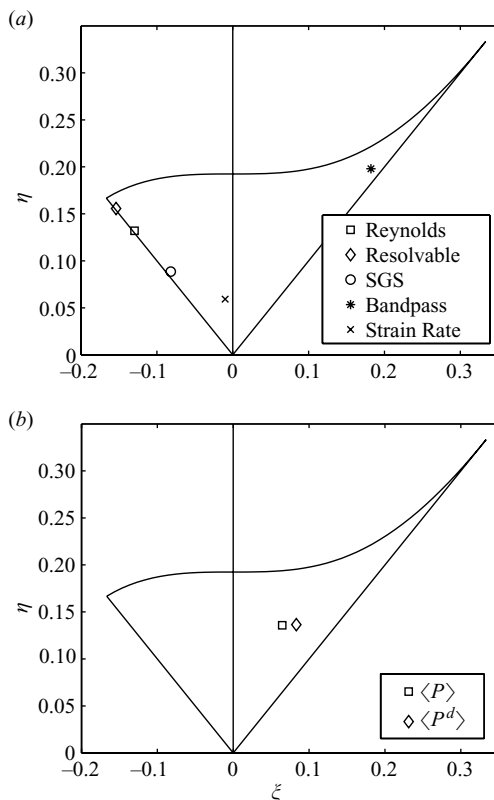
FIGURE 6. The Kosović model results ( a posteriori test) of the Lumley triangle representations of (a) the Reynolds stress, mean resolvable-scale stress, mean SGS stress, mean band-passed stress with a second filter size twice that of the first filter and the mean strain rate; (b) the mean SGS stress production rate.
