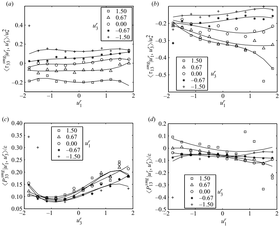
FIGURE 10. Modelled conditional SGS stress and its production rate ( a priori test) using the Smagorinsky model. Only the trend of \langle \tau_{13} | u_1^r, u_3^r \rangle is predicted reasonably well.
