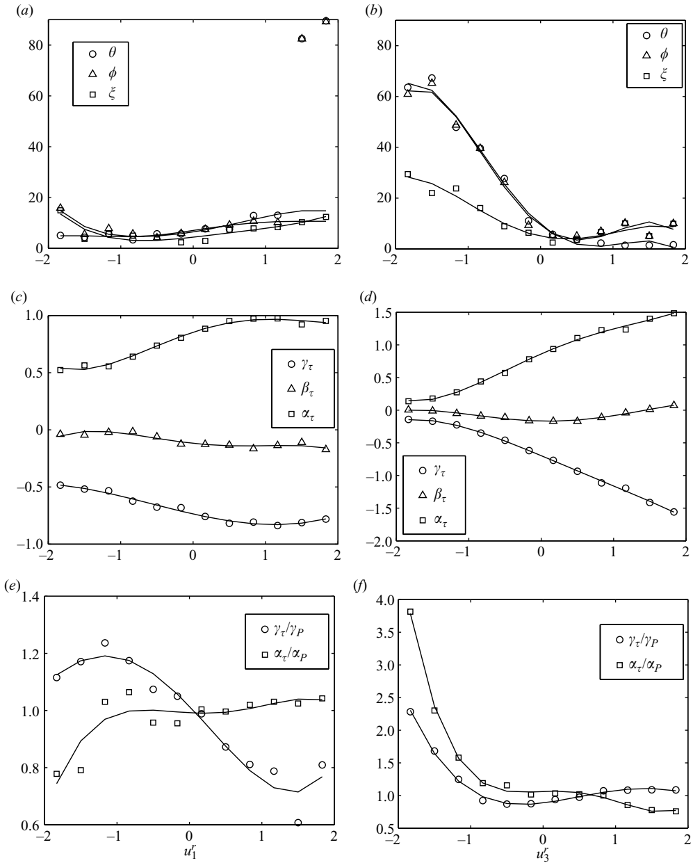
FIGURE 9. The measured geometric alignment angles and eigenvalues of the conditional SGS stress and its production rate: (a, b) the geometric alignment angles; (c, d) the eigenvalues of the conditional SGS stress; (e, f) the eigenvalue ratios of the conditional SGS stress to its production rate.
