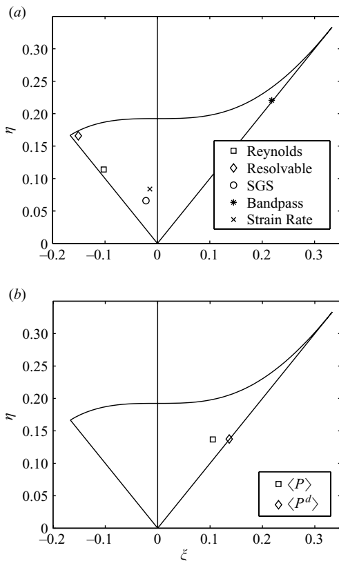
FIGURE 4. The Smagorinsky model results ( a posteriori test) of the Lumley triangle representations of (a) the Reynolds stress, mean resolvable-scale stress, mean SGS stress, mean band-passed stress with a second filter size twice that of the first filter and the mean strain rate; (b) the mean SGS stress production rate.
