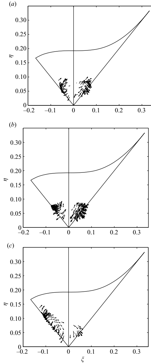
FIGURE 14. LES results ( a posteriori test) of the Lumley triangle representation of the conditional SGS stress using (a) the Smagorinsky model; (b) the split model; (c) the Kosović model.
