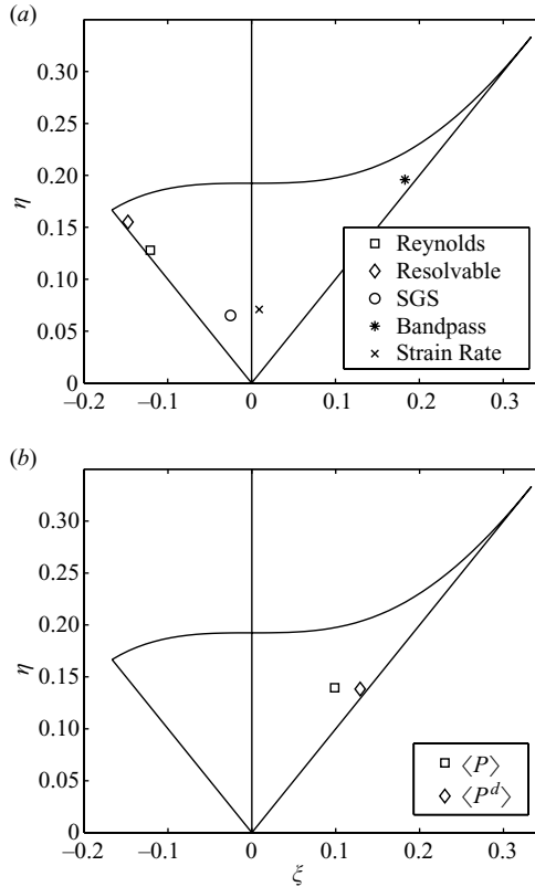
FIGURE 5. The split model results ( a posteriori test) of the Lumley triangle representations of (a) the Reynolds stress, mean resolvable-scale stress, mean SGS stress, mean band-passed stress with a second filter size twice that of the first filter and the mean strain rate; (b) the mean SGS stress production rate.
