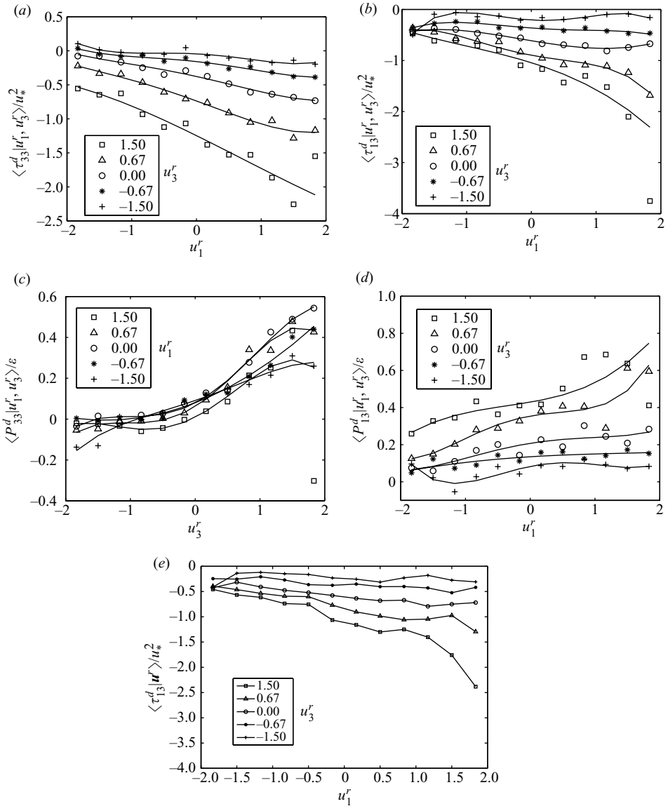
FIGURE 7. Conditional means of the measured deviatoric SGS stress components and its production rate conditional on the resolvible-scale velocity components. The dependence on the horizontal velocity components is generally stronger for positive u_3^r . The conditional shear stress component obtained using a combination of a cross-stream top-hat filter and a streamwise Gaussian filter having the same variance as the top-hat filter (e) is within 10% of that obtained using top-hat filters (b).
