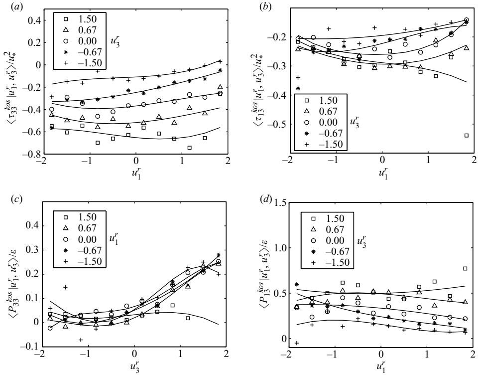
FIGURE 12. Modelled conditional SGS stress and its production rate ( a priori test) using the Kosović model.
