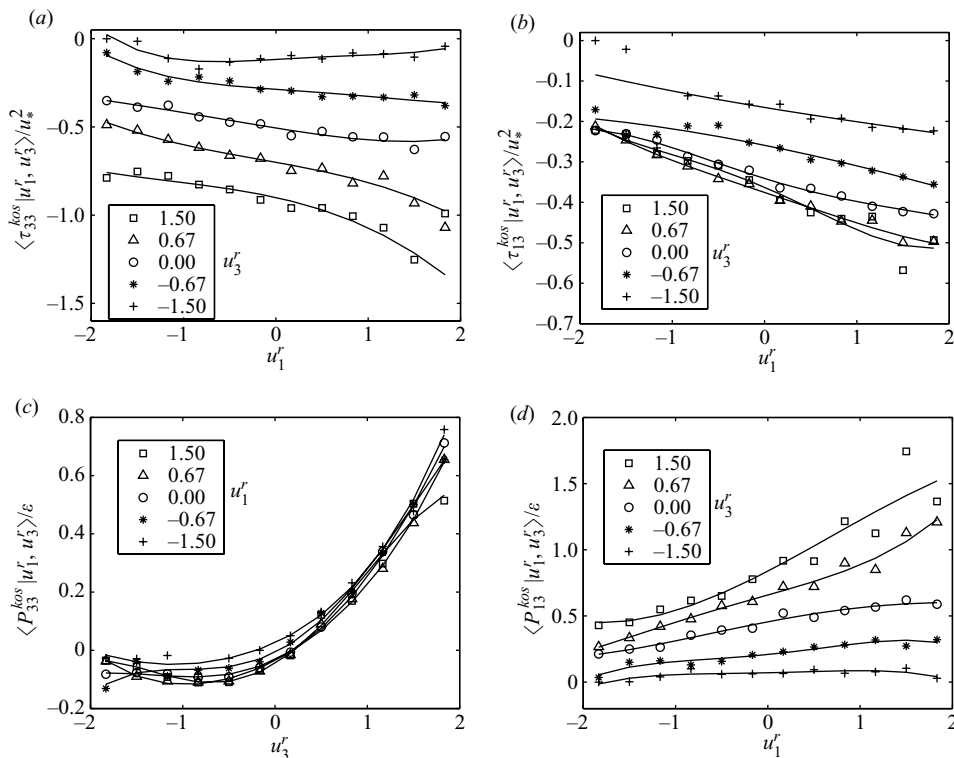
FIGURE 18. The Kosović model results ( a posteriori test) of the conditional SGS stress and its production rate.
