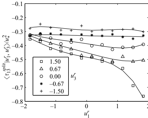
FIGURE 11. Modelled conditional SGS shear stress ( a priori test) using the split model. The variations of the predicted \langle \tau_{13} | u_1^r, u_3^r \rangle are smaller but the magnitude is larger than that of the Smagorinsky model due to the contribution from the mean part.
